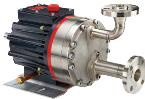
G25 with Stainless Steel pump head and ANSI RF flanges.
